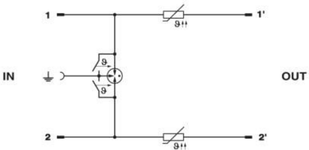
Circuit diagram
