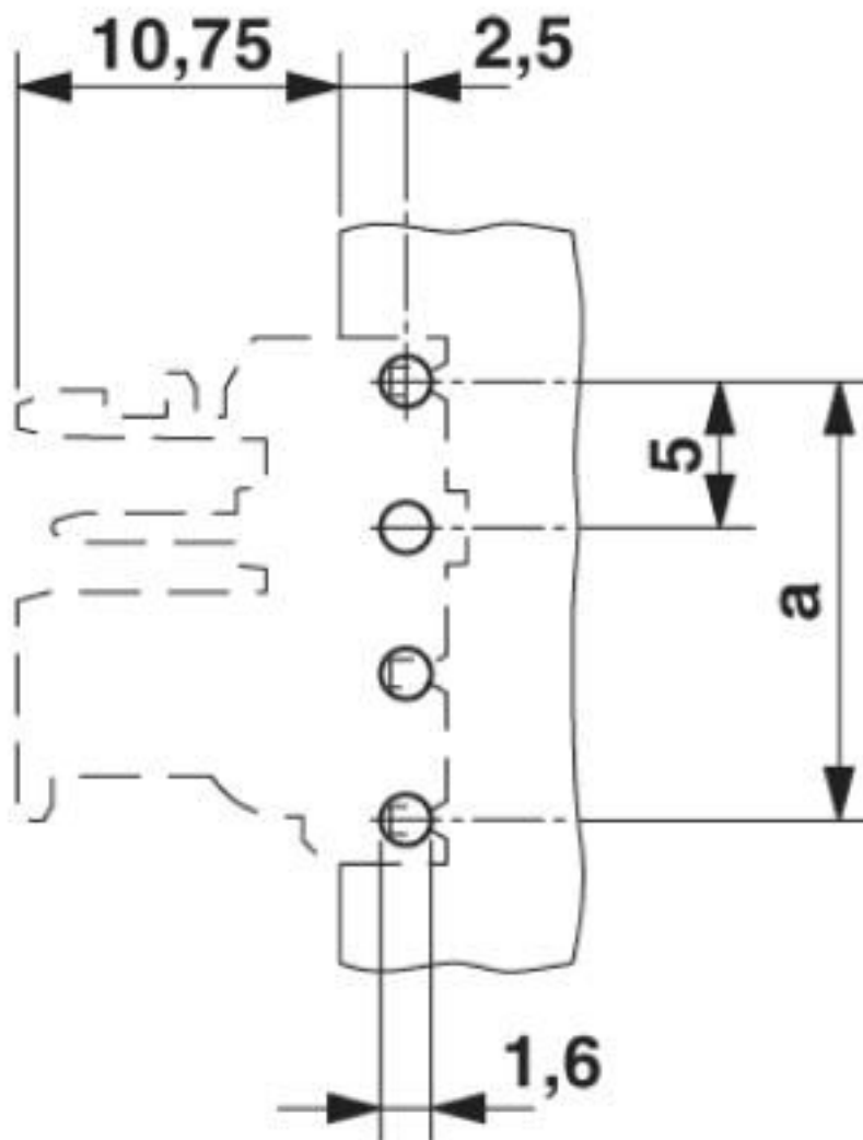
Drilling diagram
