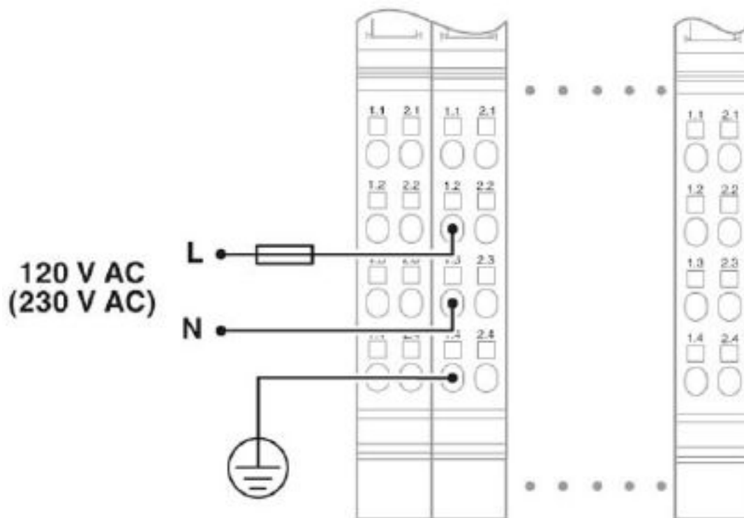
Connection diagram
