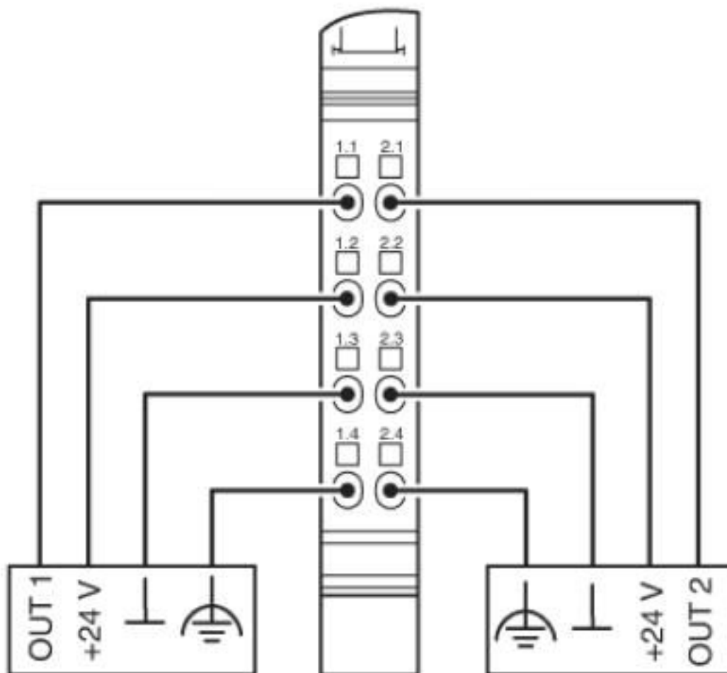
Connection diagram
