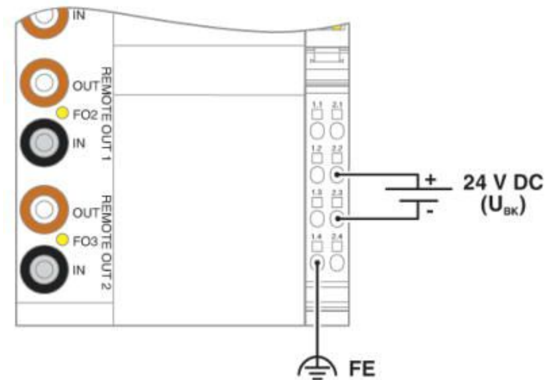
Connection diagram
