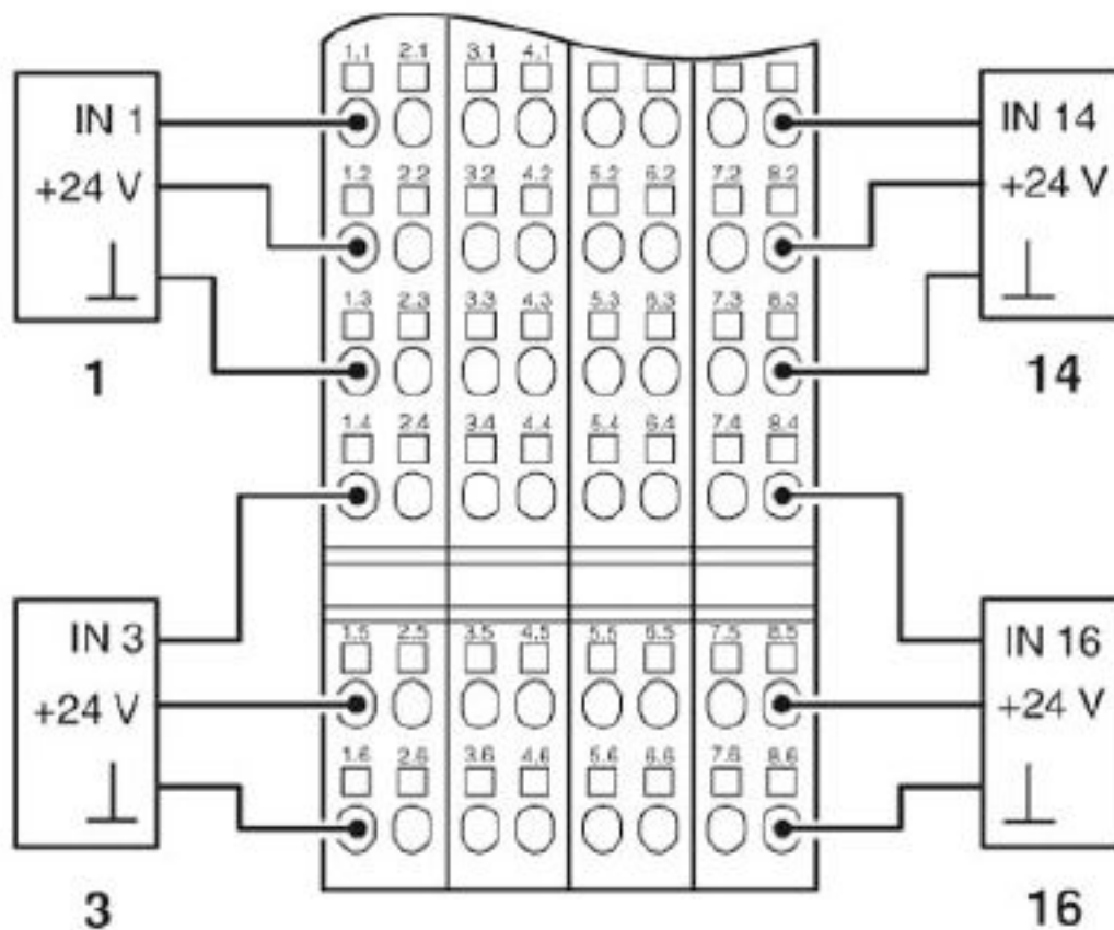
Connection diagram
