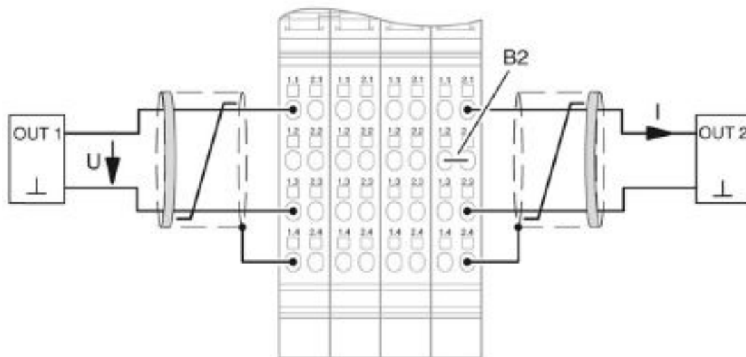
Connection diagram
