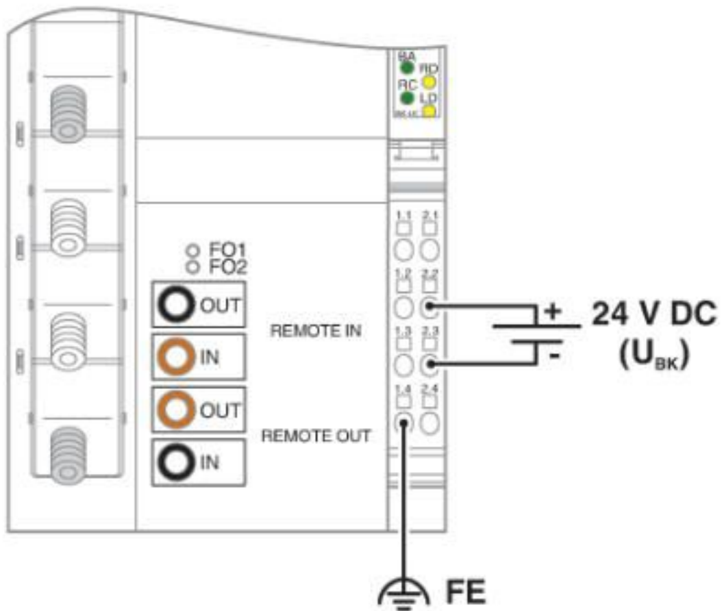
Connection diagram
