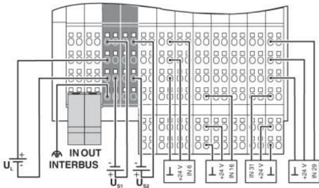
Connection diagram
