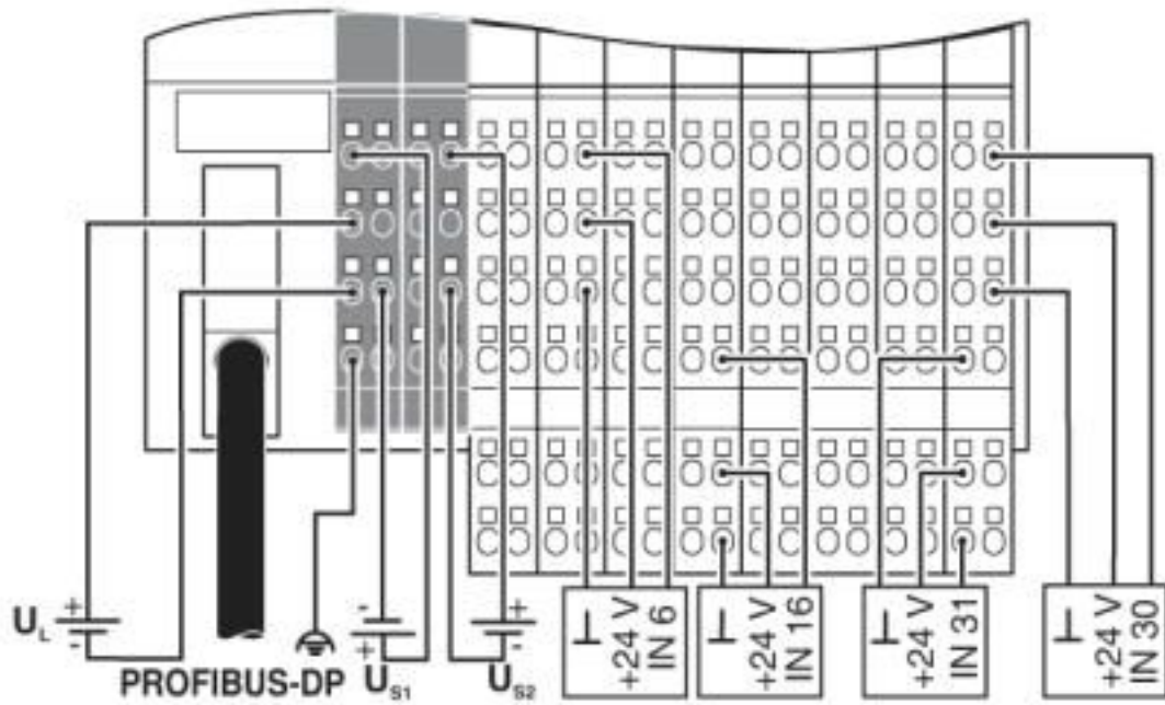
Connection diagram
