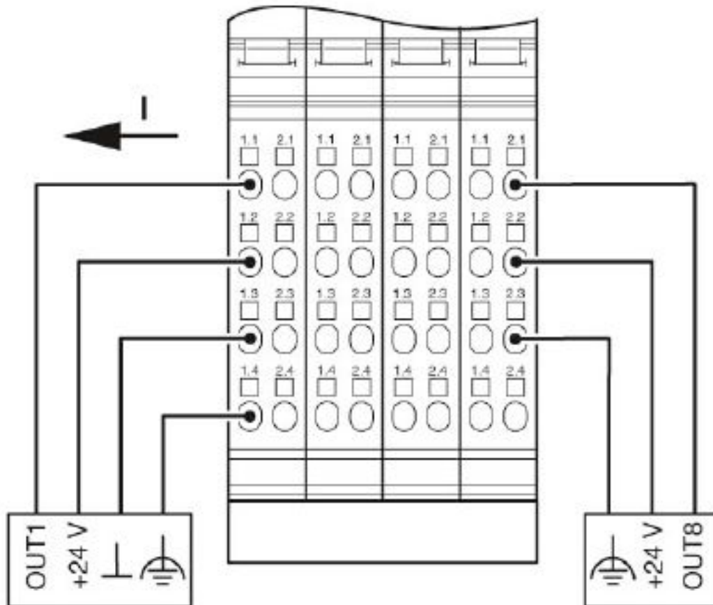
Connection diagram
