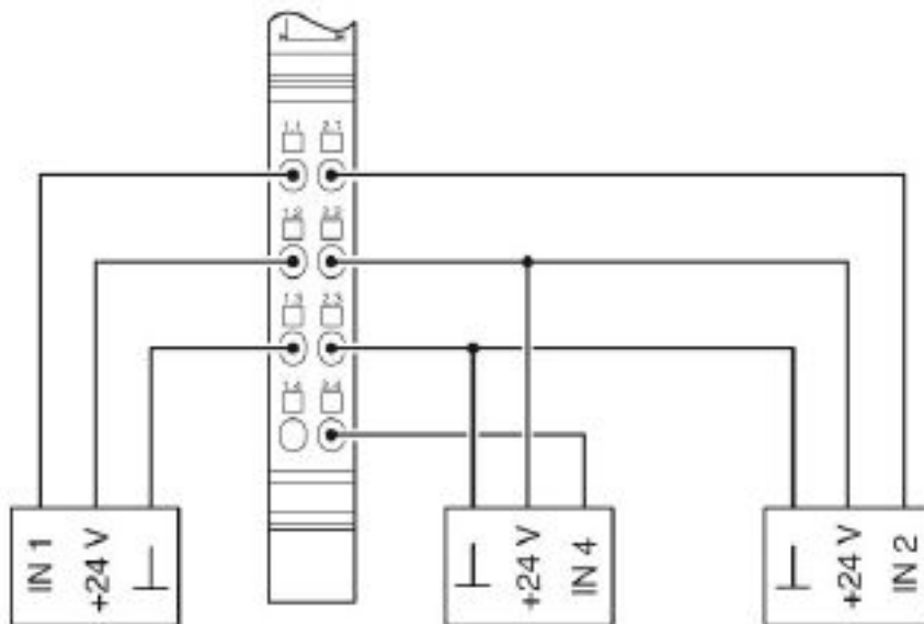
Connection diagram
