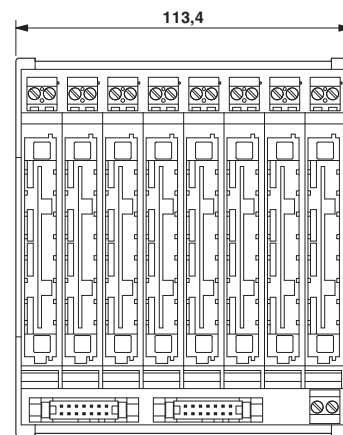
Dimensional drawing
