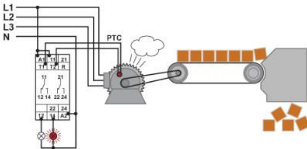
Application drawing
