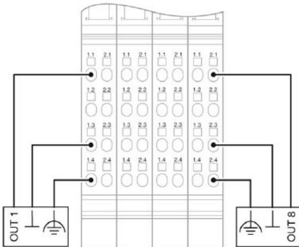
Connection diagram
