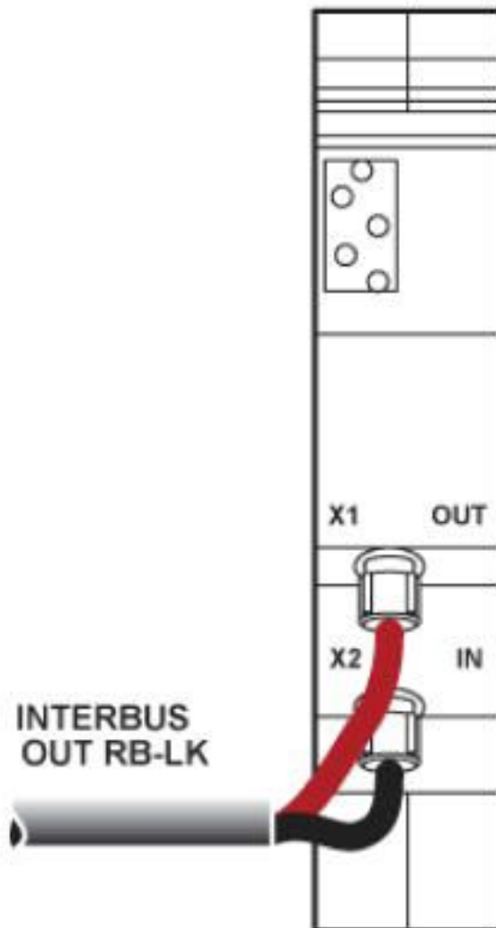
Connection diagram
