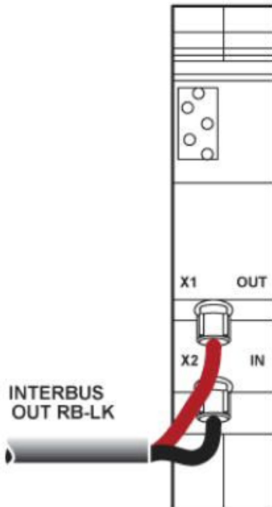
Connection diagram
