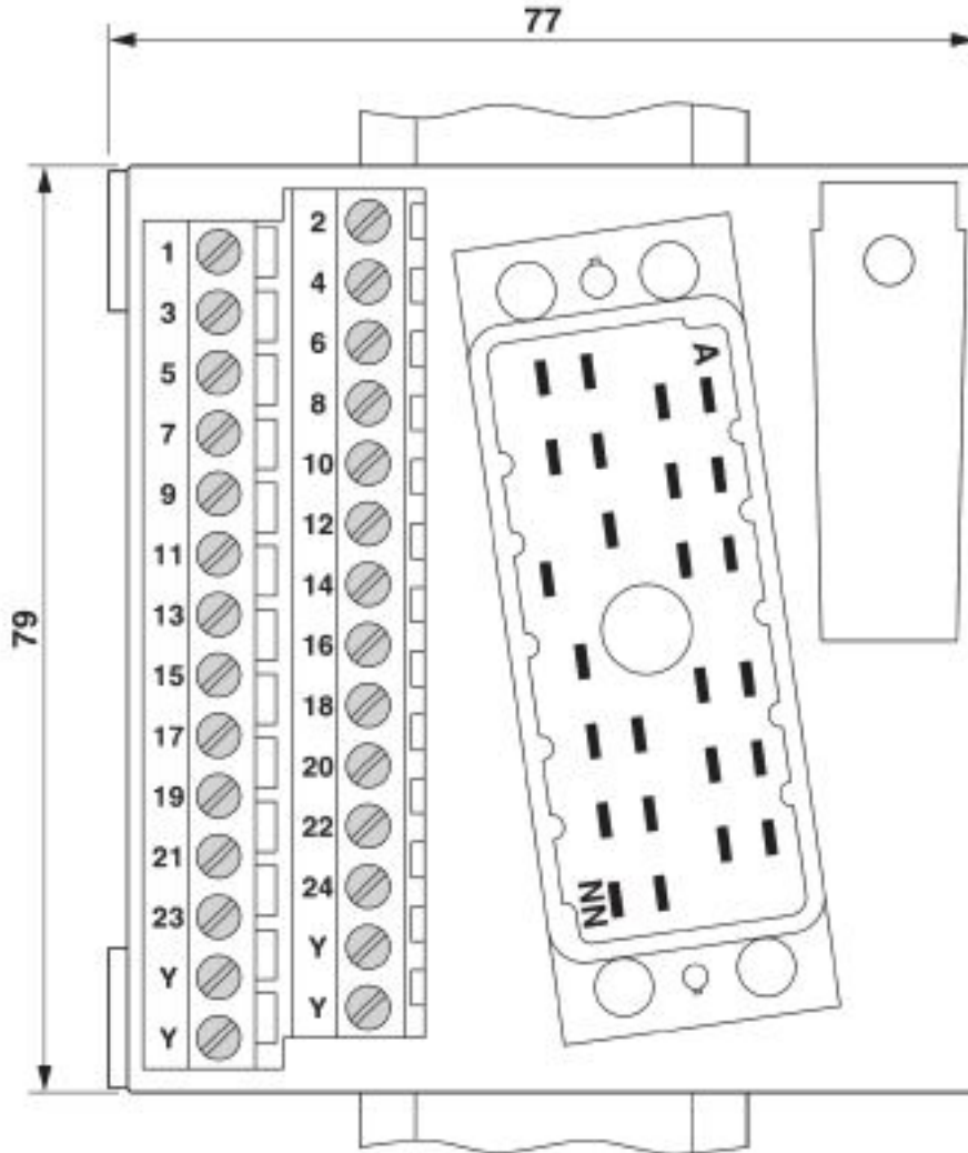
Dimensional drawing
