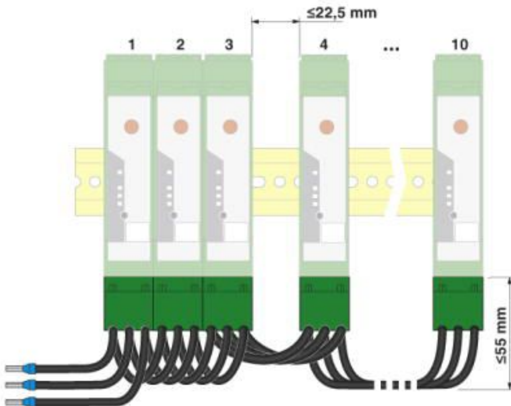
Application drawing
