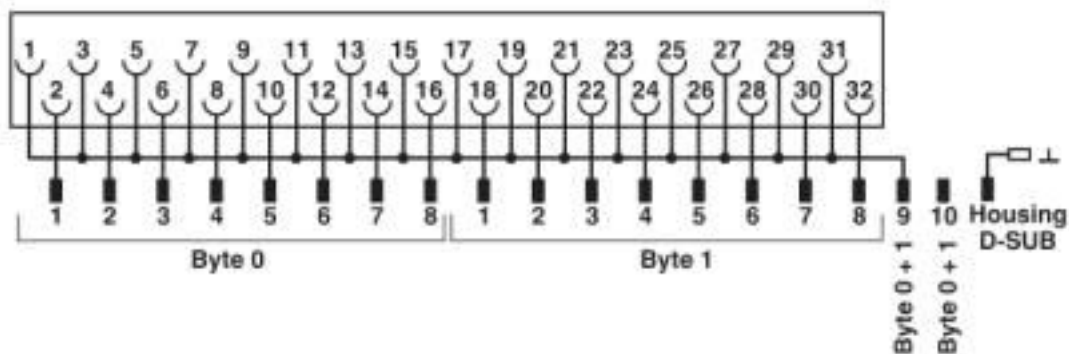
FLKM-PA-2D15/HW/DI/C300 connection scheme
