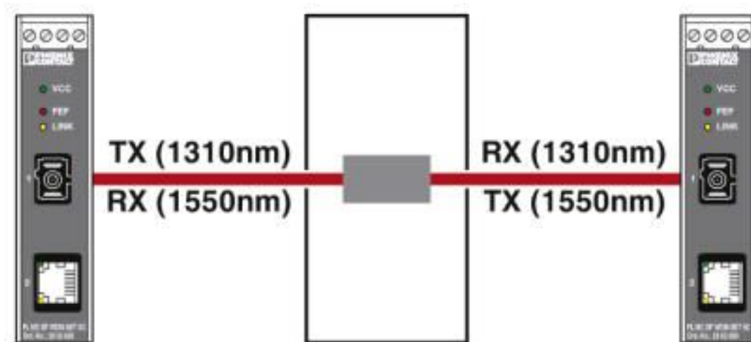
Application drawing
