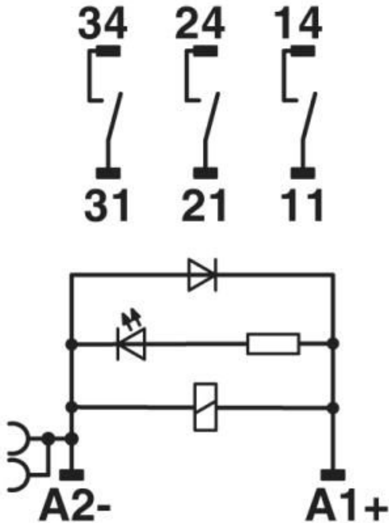
Circuit diagram
