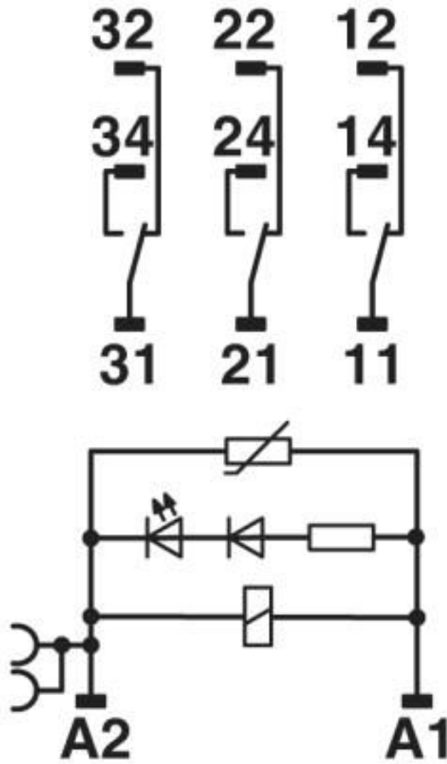
Circuit diagram
