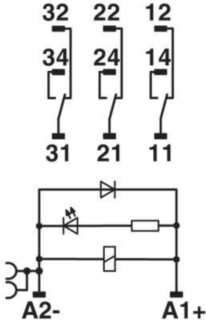
Circuit diagram
