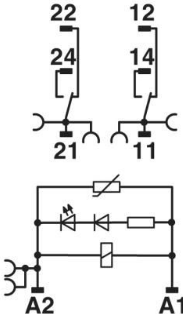
Circuit diagram
