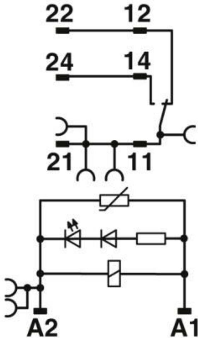
Circuit diagram
