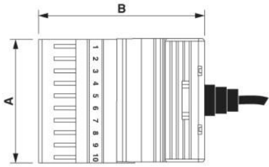
Dimensional drawing
