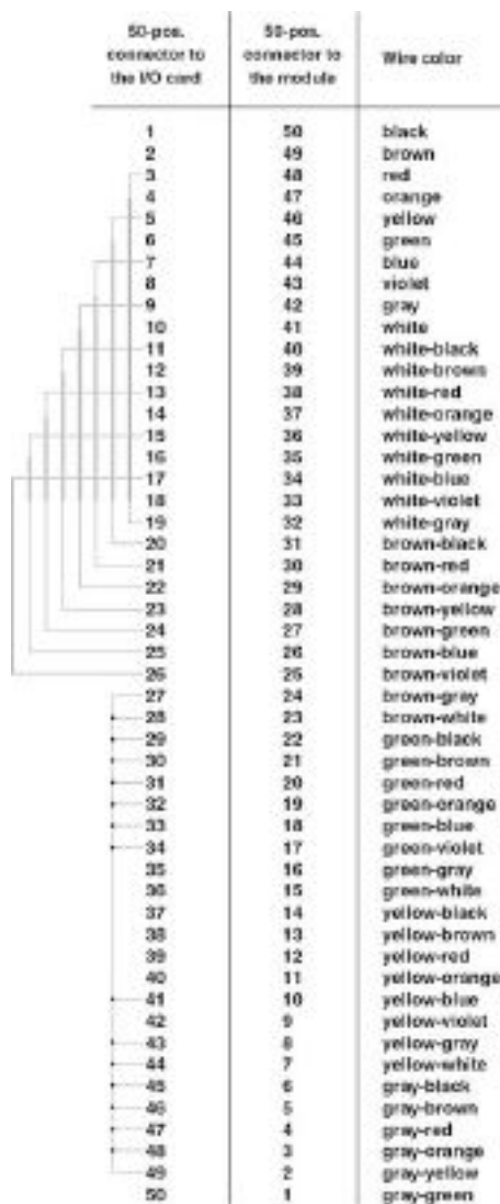
Connection diagram
