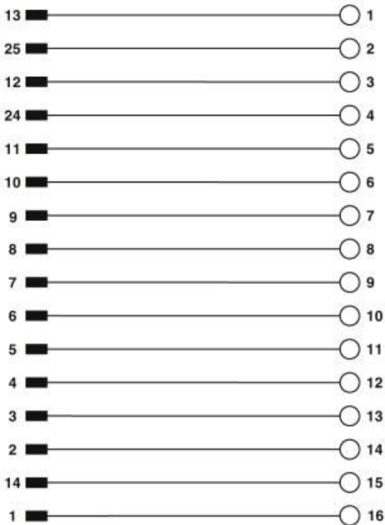
Circuit diagram
