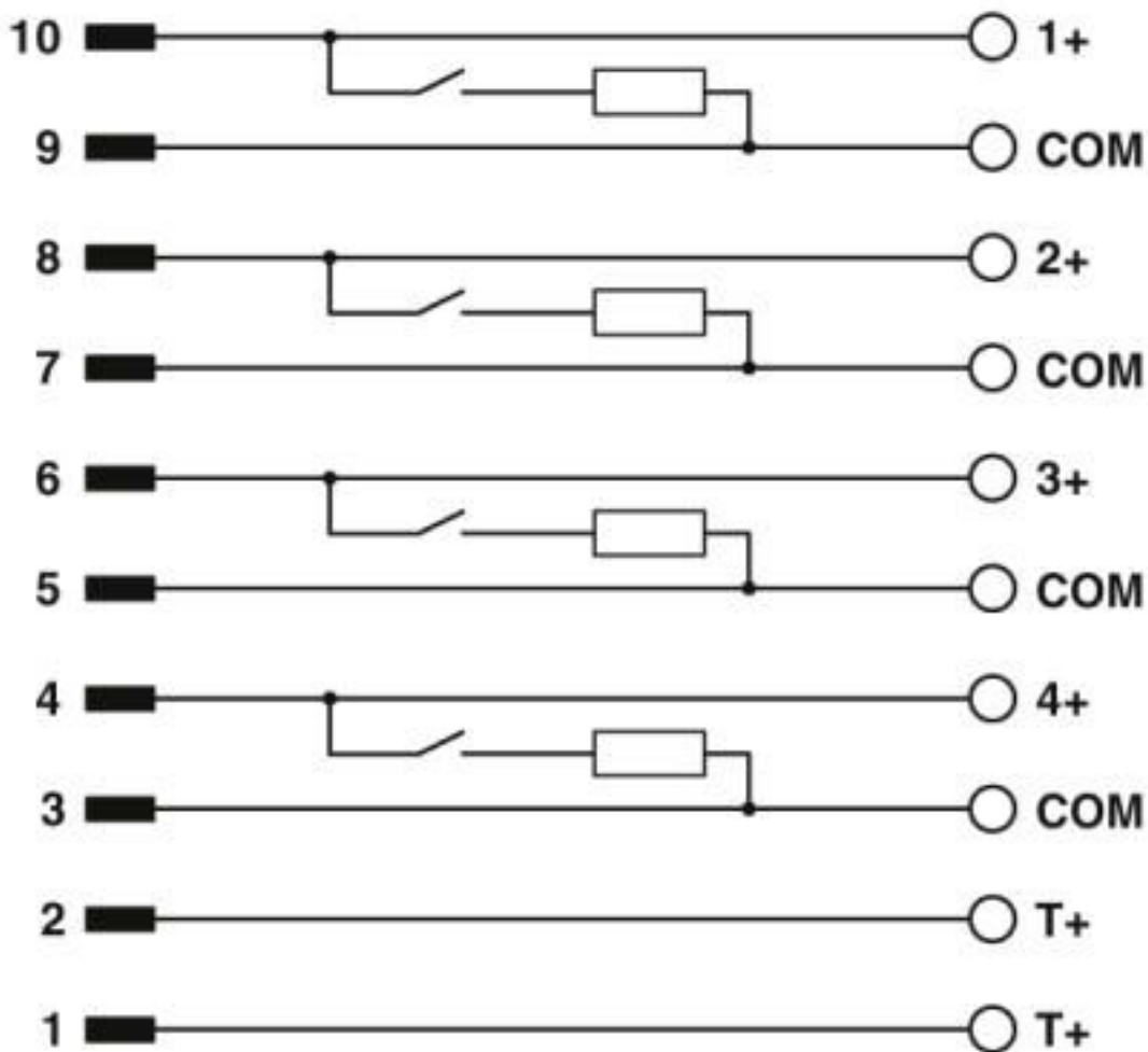
Circuit diagram
