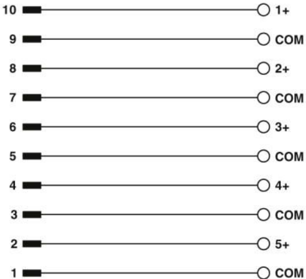
Connection scheme VIP-2/.../FLK50 (1-40) /S7
