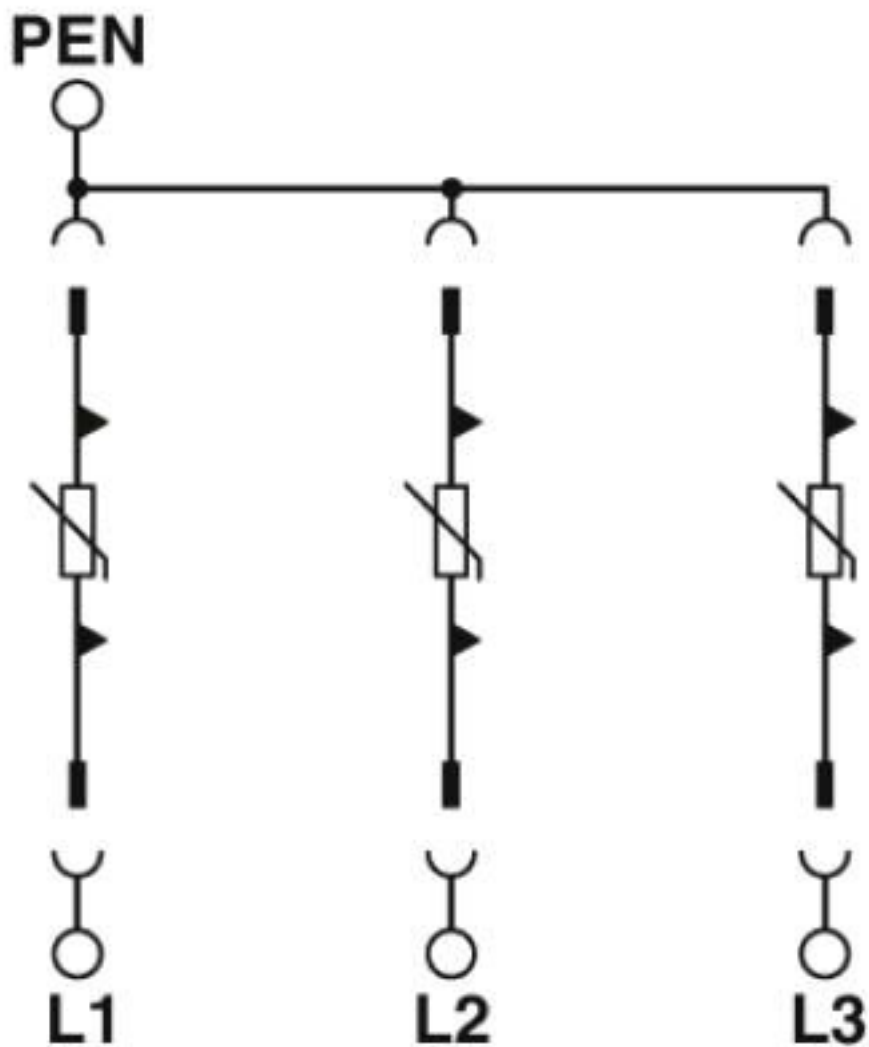
Circuit diagram
