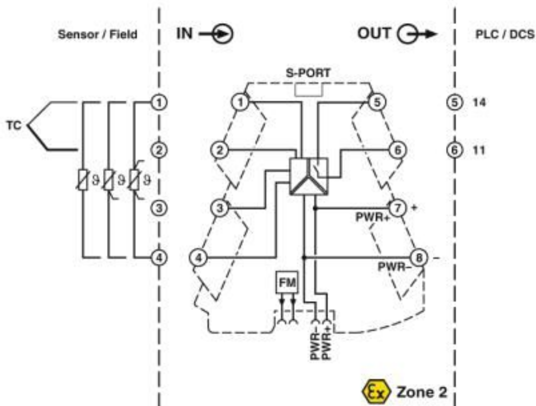
Block diagram
