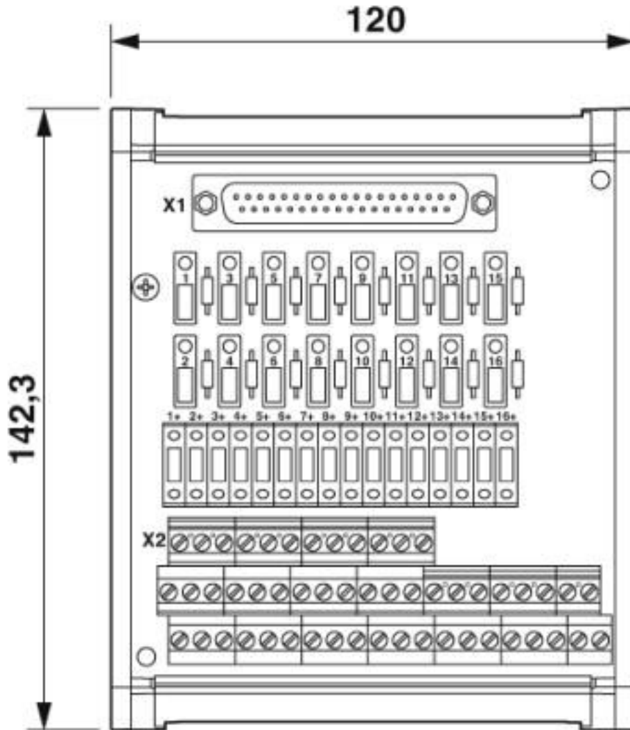
dimensional drawing of left hand version
