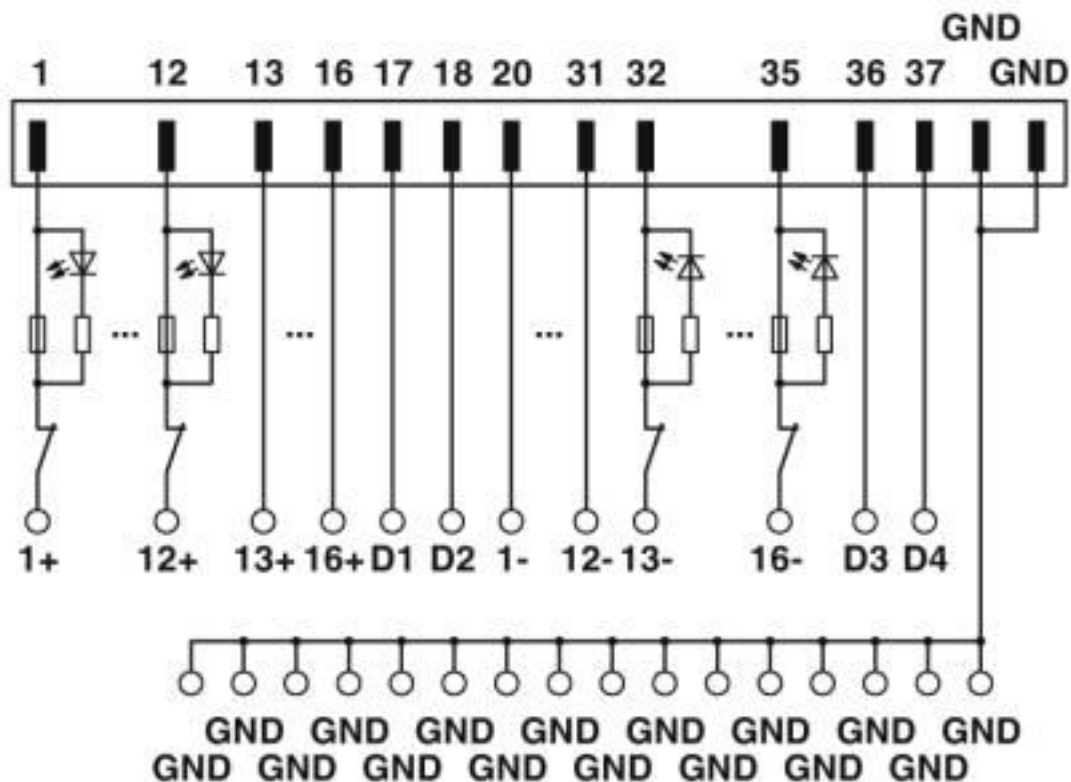
Circuit diagram
