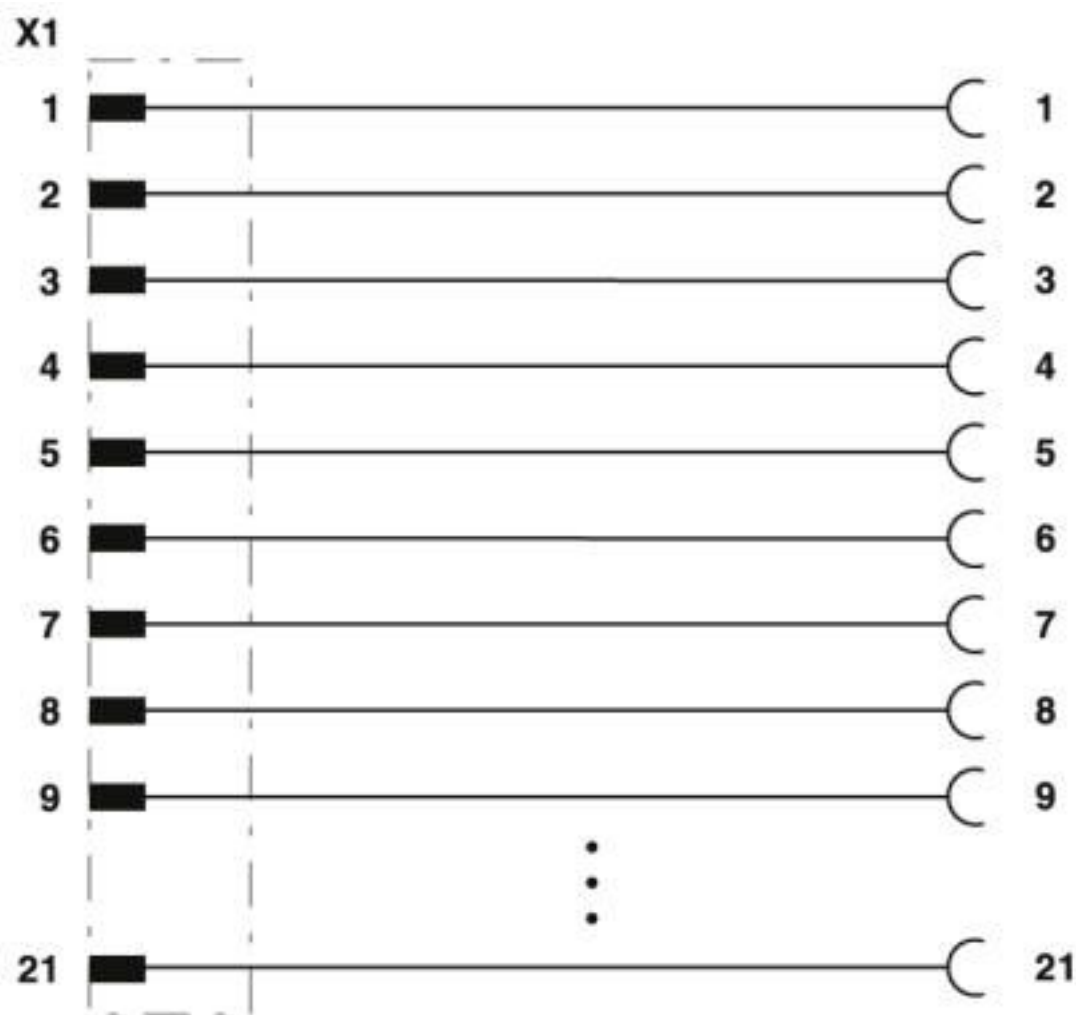
Circuit diagram
