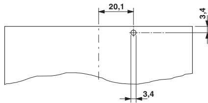
Drilling diagram
