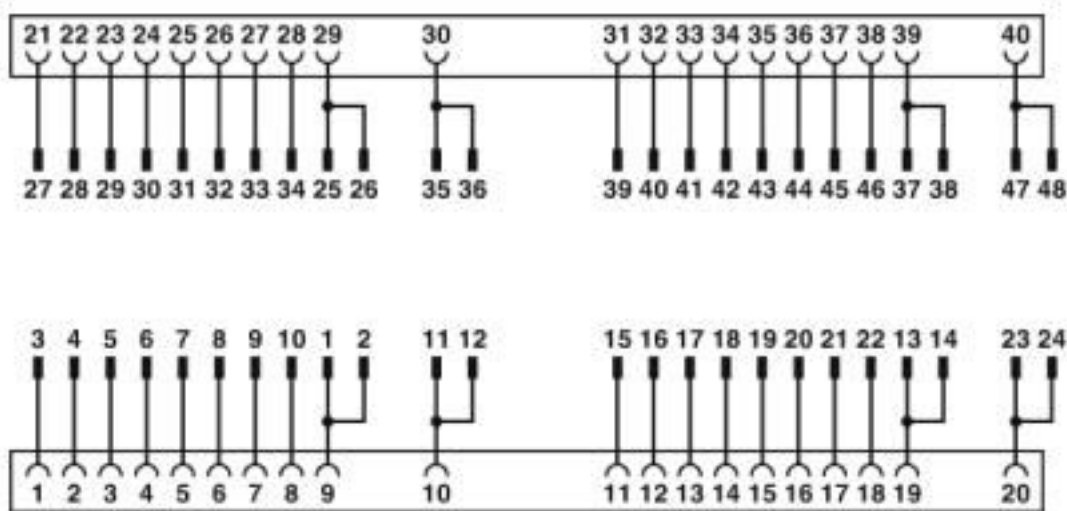
Connection scheme FLKM 50-PA/AN/S7-1500
