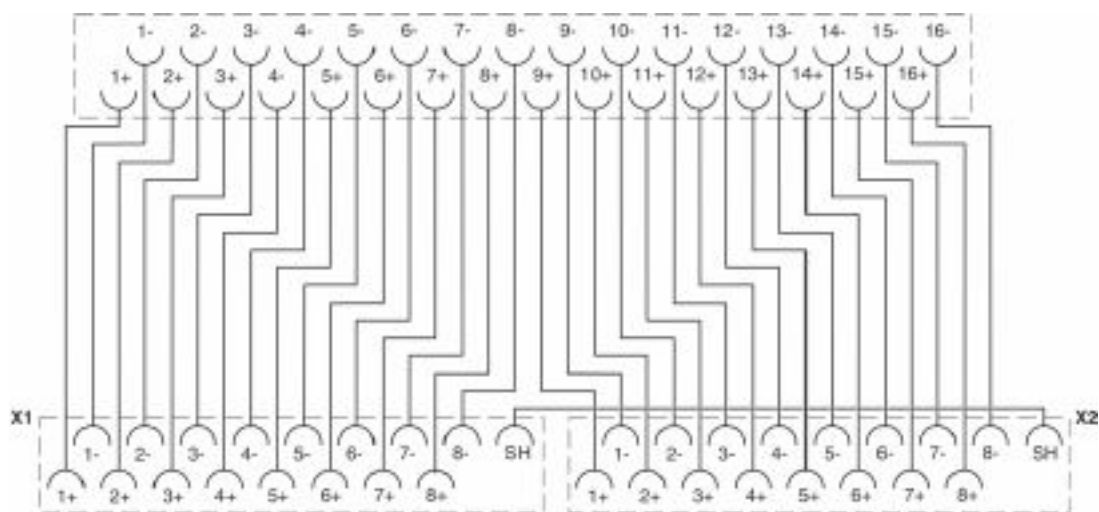
Circuit diagram
