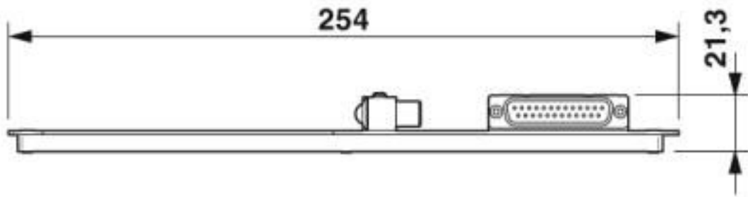
Dimensional drawing
