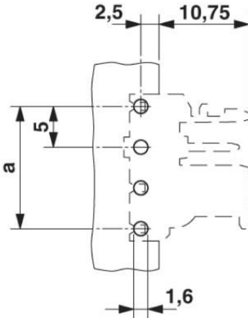
Drilling diagram
