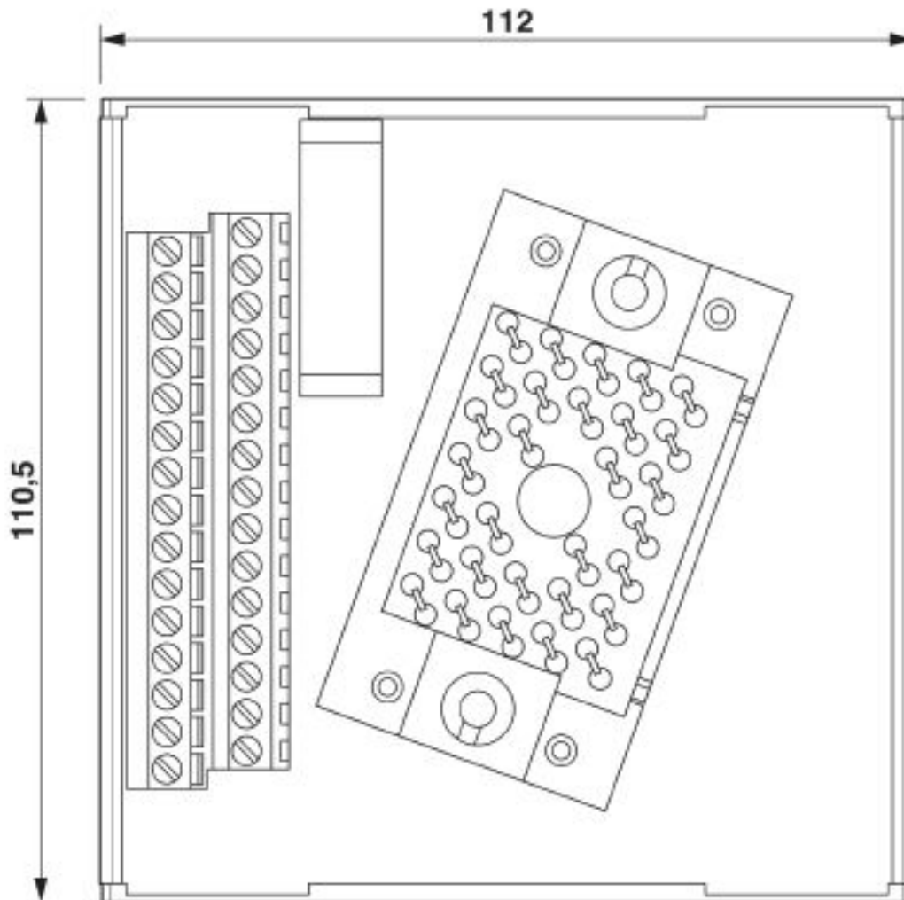
Dimensional drawing
