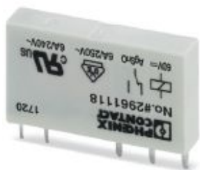
Plug-in miniature power relay, with power contact, 1 PDT, input voltage 60 V DC
