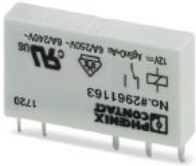
Plug-in miniature power relay, with multi-layer gold contact, 1 PDT, input voltage 12 V DC
