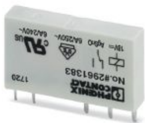
Plug-in miniature power relay, with power contact, 1 PDT, input voltage 18 V DC
