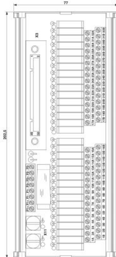
Dimensional drawing
