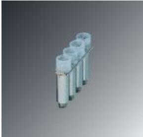
Fixed bridge, pitch: 5 mm, number of positions: 4, color: silver
