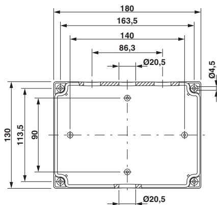
Dimensional drawing
