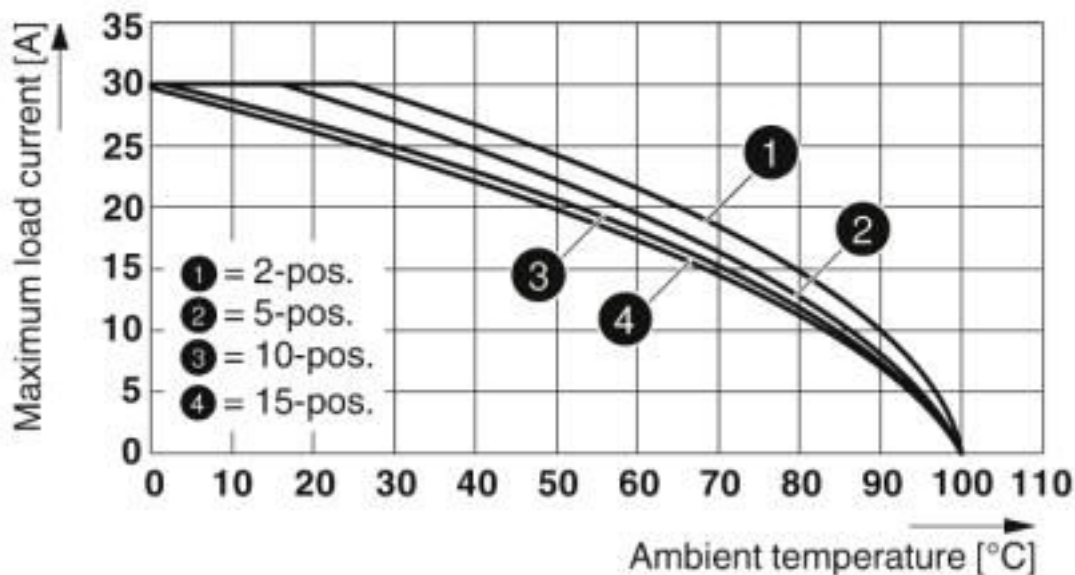
Derating curve for ST 4/ 1P and for all plug versions SP...
