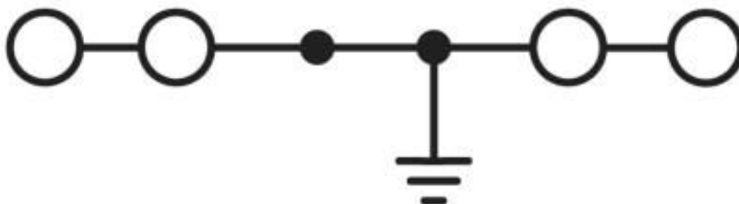
Circuit diagram
